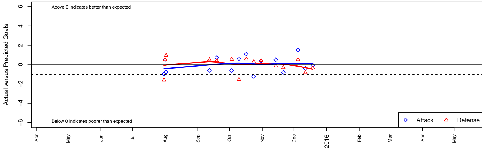
Storm King G01 Dots are actual minus expected GF (blue circles) and GA (red triangles). Blue line is smoothed change in attack strength. Red is smoothed change in defense strength.
